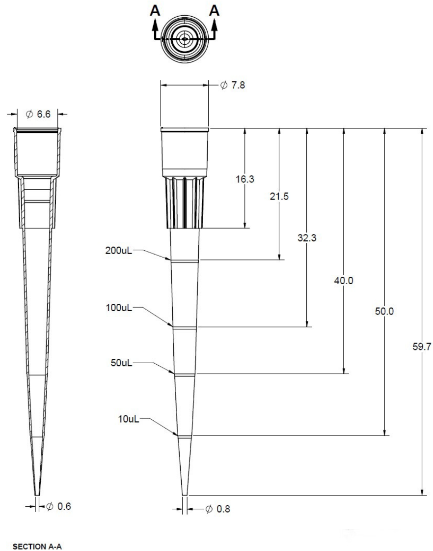
WB 6650 TripleA 300uL LTS®-Compatible Tips Eco Refill – Non filtered
